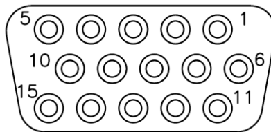
MATING FACE
